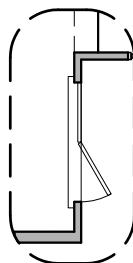
Center Hinge ILO Sliding Glass Door
